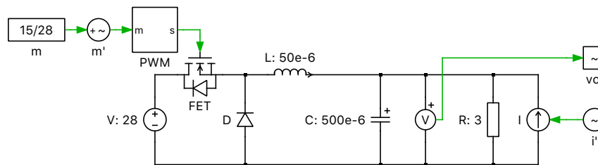
Figure 1: Buck converter with analysis tools
