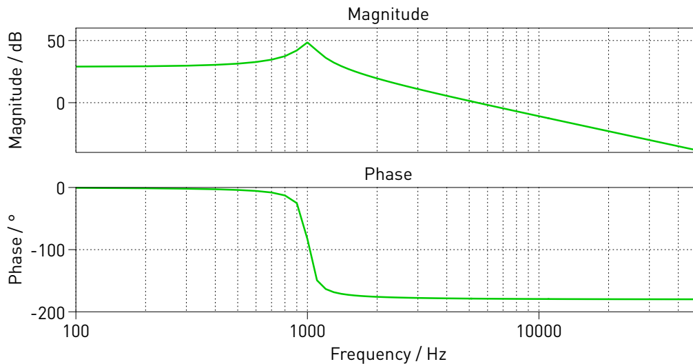
Figure 2: Control-to-output transfer function of open loop buck converter
