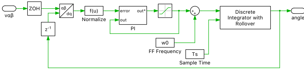
Figure 2: Synchronous reference frame phase-locked loop (SRF-PLL)
