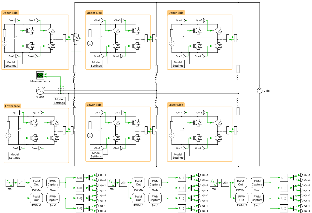
Figure 2: Schematic of the grid-connected MMC inverter
