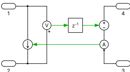
Figure 4: Circuit to allow physical system splitting
