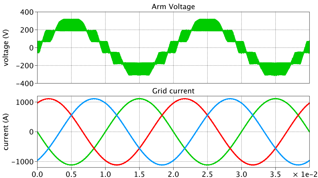
Figure 5: Real-time measurements obtained on the RT Box in multi-tasking mode
